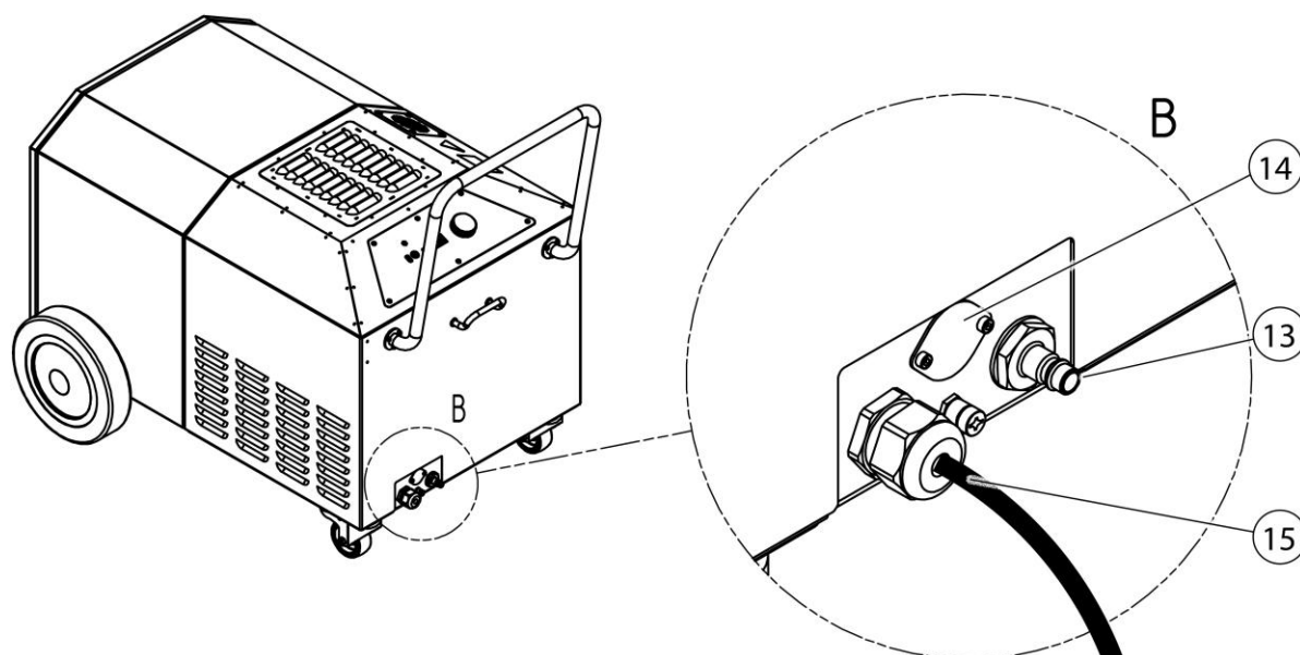
Fig. 2: Connections
